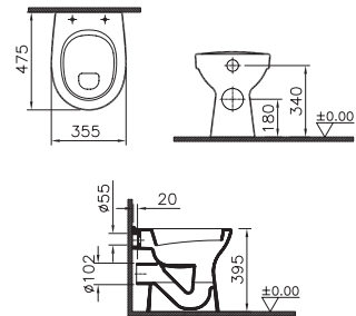
Stand-Flachspül-WC 355 x 395 x 475 mm
