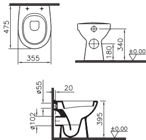
Stand-Tiefspül-WC* 355 x 395 x 475 mm
